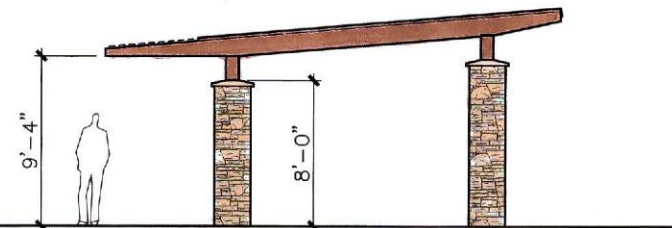
SMALL SHELTER SIDE ELEVATION
