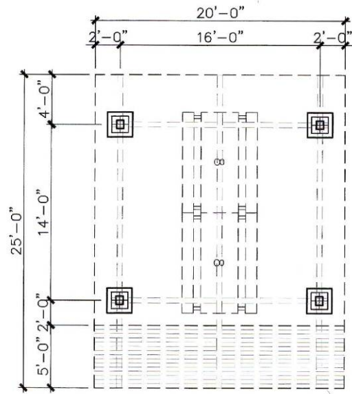
SMALL SHELTER PLAN
