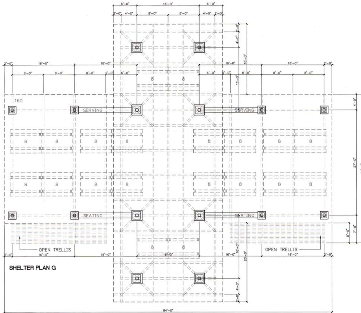
BLACK HOOF PARK – PHASE II LARGE SHELTER PLAN
