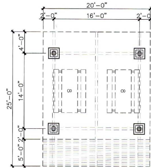
SMALL SHELTER PLAN - SEATING ALT.
