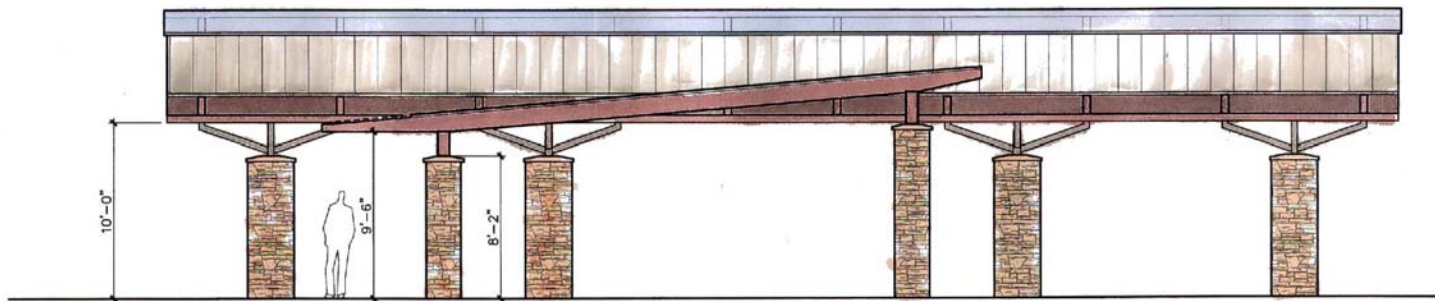
SIDE ELEVATION
