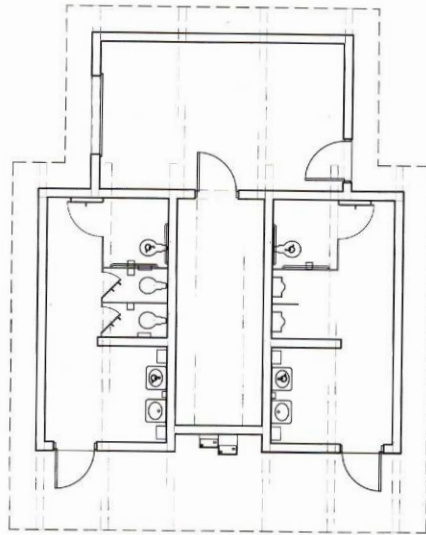
TOILET PLAN B - WITH ALTERNATE STORAGE
